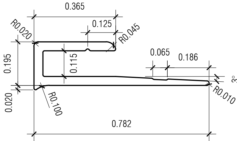
1 SIDE VIEW scale: NTS
