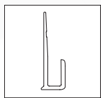
AP-50 Bullnose Cap for .150" Panel
