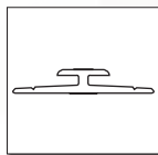
FR-0431AN12* Slim-Division Bar Trim for .150" Panel (.437" face)
