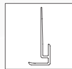
FR-0431AN12* Slim-Division Bar Trim for .150" Panel (.437" face)
