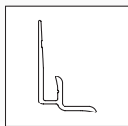
AP-32 Inside Corner and Cove for .150" Panel
